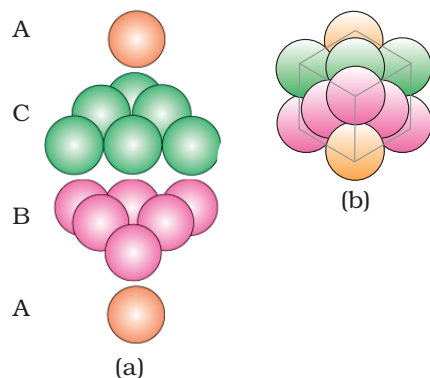
Fig. 1.19 (a) ABCABC... arrangement of layers when octahedral void is covered (b) fragment of structure formed by this arrangement resulting in cubic close packed (ccp) or face centred cubic (fcc) structure.
