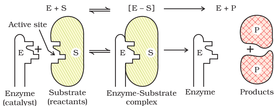
Fig. 5.4: Mechanism of enzyme catalyzed reaction
