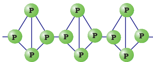
Fig.7.3: Red phosphorus
