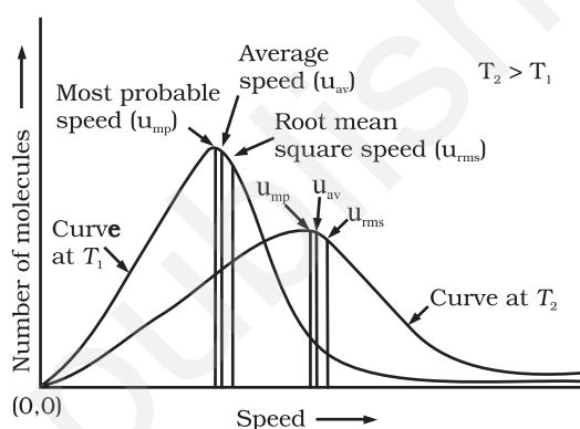
Fig. A(1) : Maxwell-Boltzmann distribution of speeds
